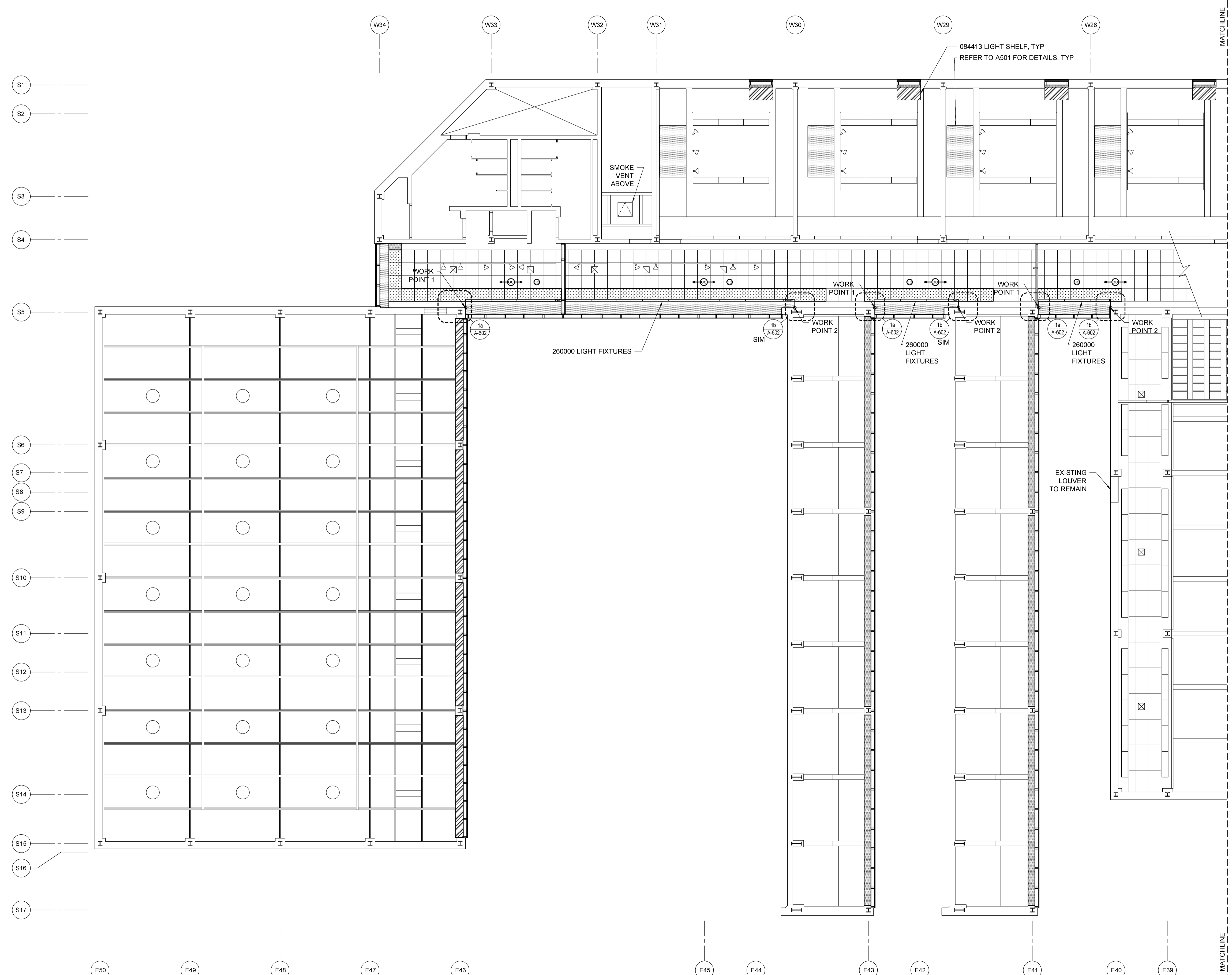
1 LEVEL 2 REFLECTED CEILING PLAN SCALE: 1/8" = 1'-0"
