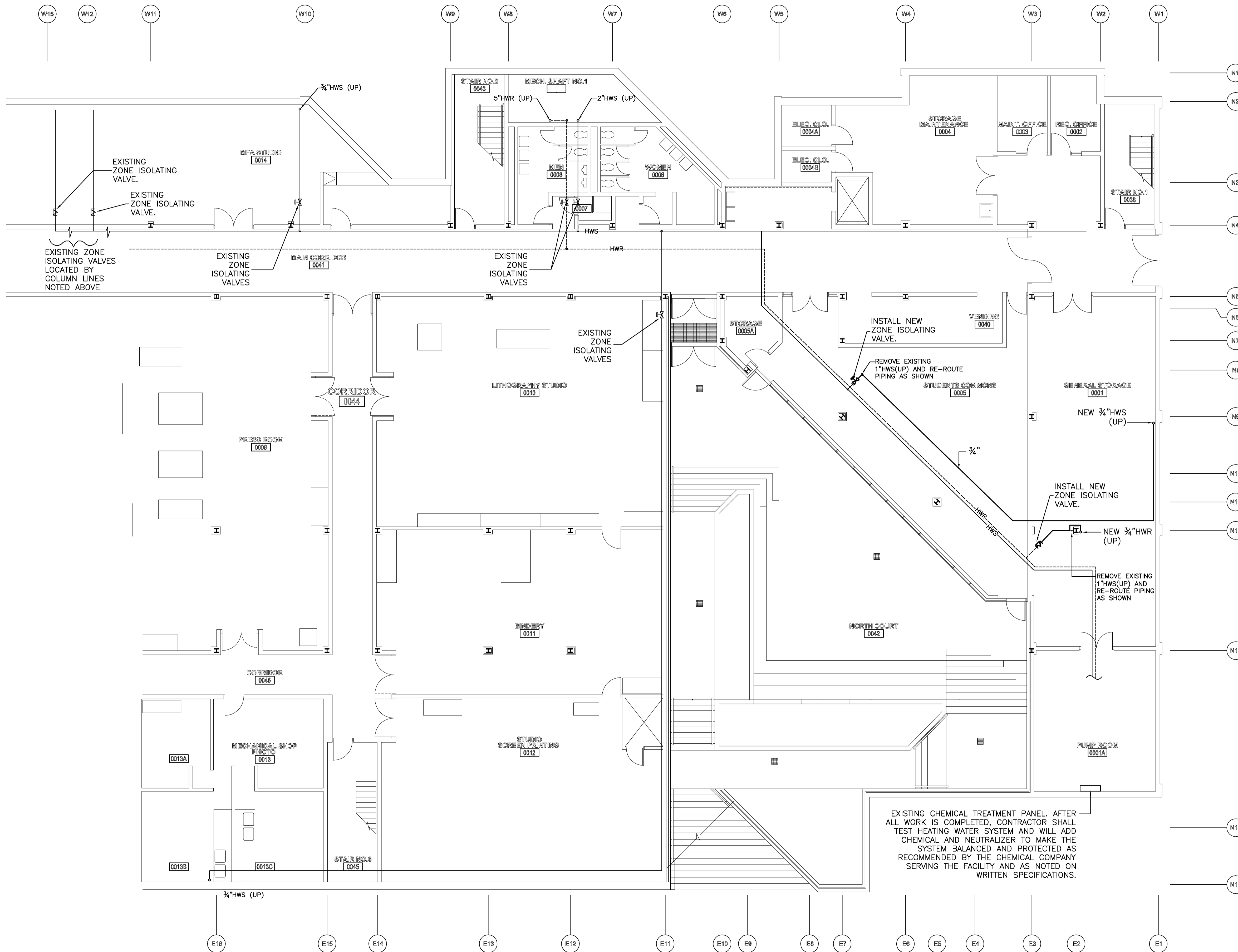
BASEMENT FLOOR PLAN SCALE: 1/8" = 1'-0"
